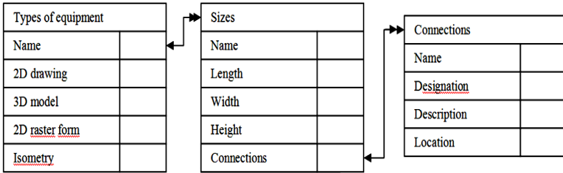
Fig 11.1. The structure of the equipment database
