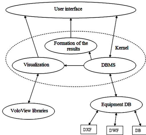
Fig. 11.2. The structure of electronic databanks
